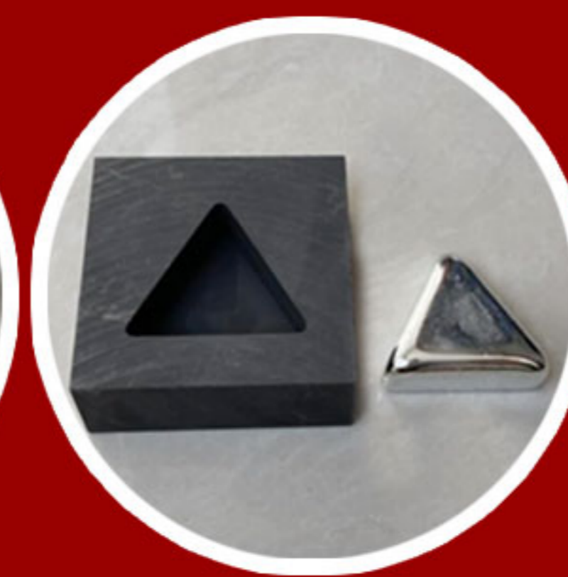
Metal Mold
